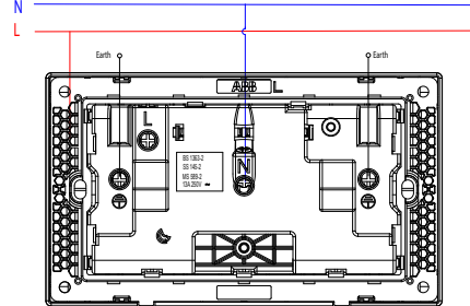
2G 13 A switched socket outlet
