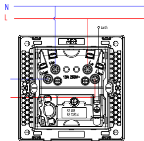
Fused switched connection unit
