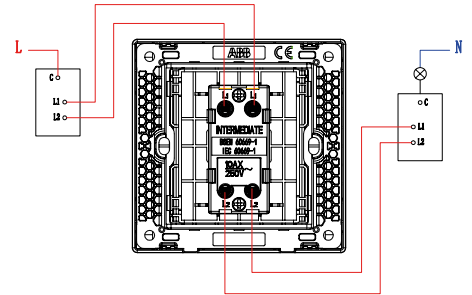
1G intermediate switch
