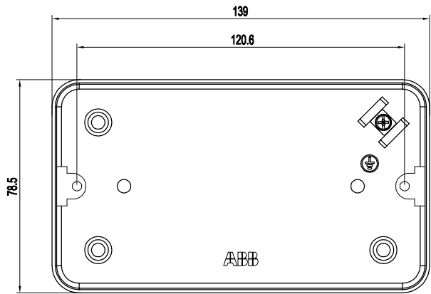
Dimensions for 2 gang mounting box
