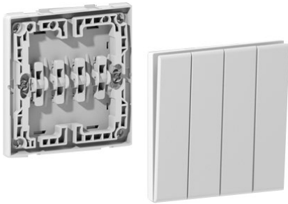
Rapid Installation with Monobloc rocker up to 4G
